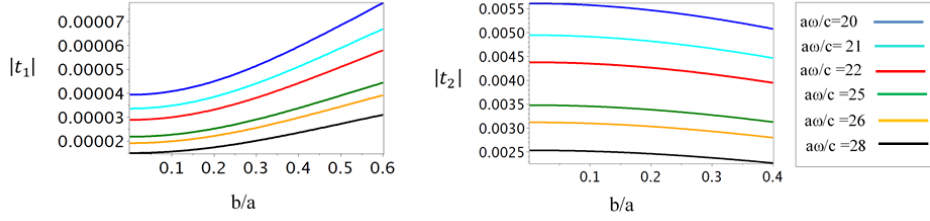
Figure 3: The magnitude of the transmission coefficients of the dominate modes ( n' = 1 ) and first produced mode ( n' = 2 ) of the output wave from the plasma the radius of the plasma valve and the incident wave frequency.
